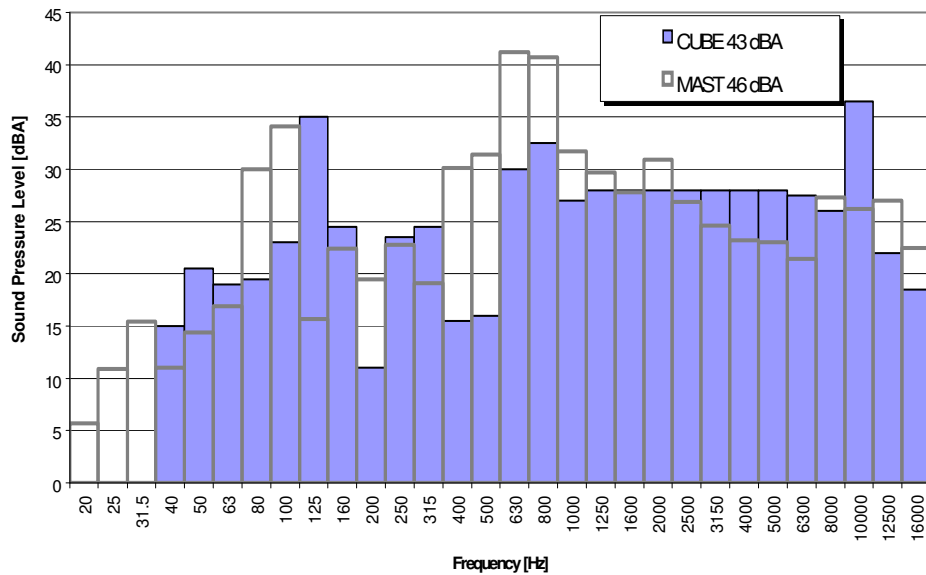
Figure 4: Spectrum of noise measured with CUBE energized and vibration up to 250 Hz. OASPL = 46 dBA.
