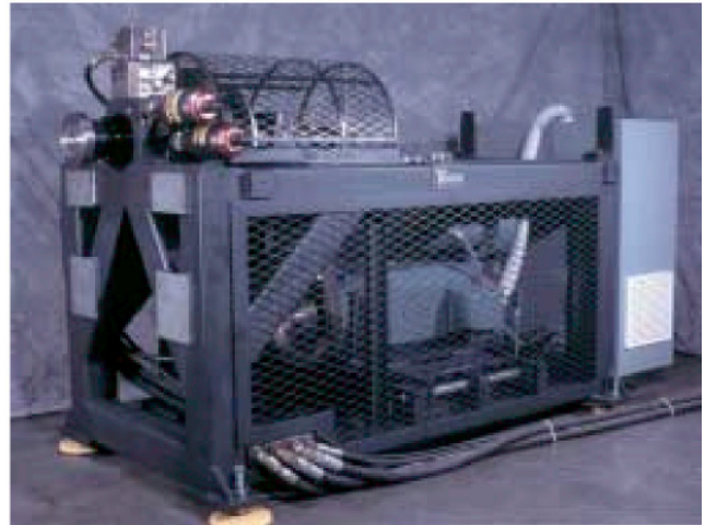
A typical Team Engine Simulation System with integrated variable speed drive.
