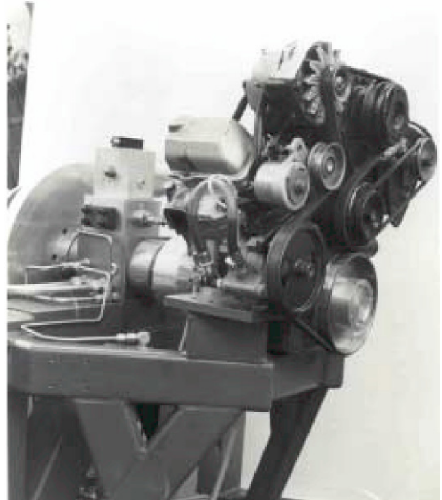
A belt test setup on an early Team Engine Simulation System.
