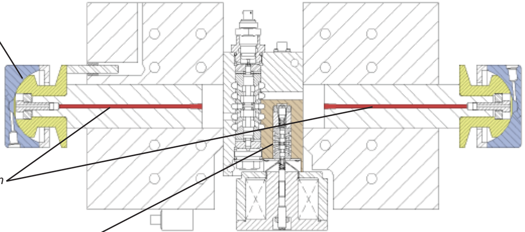
Cross Section through Team's patented Integrated Actuator®.
